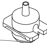
1011C1-19020 PICK-UP NOZZLE (ID = \phi 1.0, OD = \phi 1.3) KME, CM92-MT
