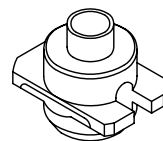
1011C1-19080 PICK-UP NOZZLE (ID = \phi 2.5, OD = \phi 3.0) KME, CM92-MT
