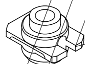
1011C1-19040 PICK-UP NOZZLE (ID = \phi 2.5, OD = \phi 4.0) KME, CM92-MT
