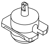
1011C1-19010 PICK-UP NOZZLE (ID = \phi 0.7, OD = \phi 1.3) KME, CM92-MT
