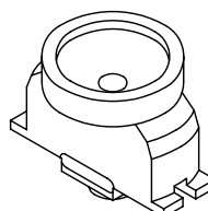
1011C1-19130 PICK-UP NOZZLE (ID = \phi 10.0, OD = \phi 12.5) KME, CM92-MT
