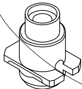
1011C1-19050 PICK-UP NOZZLE (ID = \phi 3.8, OD = \phi 4.5) KME, CM92-MT
